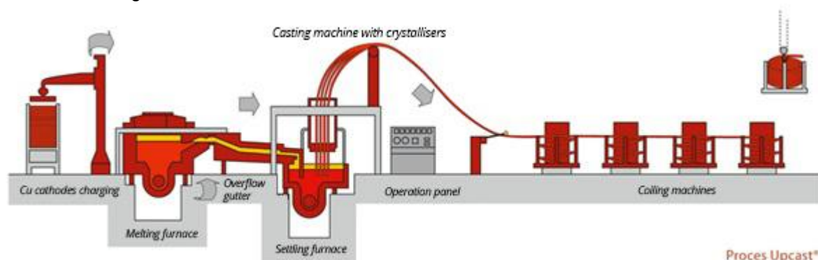
Schematic representation of the UPGAST process used for the production of Cu-OFE oxygen-free copper wire at the Cedynia Copper Wire Rod Plant Division.
