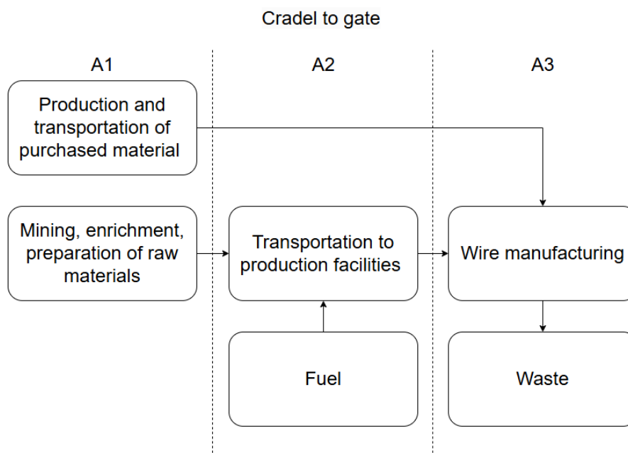
Cradle-to-gate process flow diagram for Copper OFE Wire production, including modules A1–A3.
